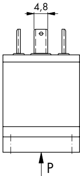
Pressure connections on subplate.
