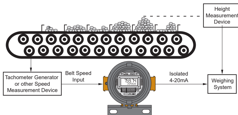
Figure 6. Used in conjunction with a weighing system, the FDY can be used for conveyor belt weight calculations
